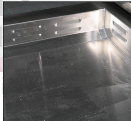
Unique MEDIS MT Side Wall Downdraft Extraction System (Standard Feature). Note: there is no air extraction opening in the plenum of the large sink below the work area!
