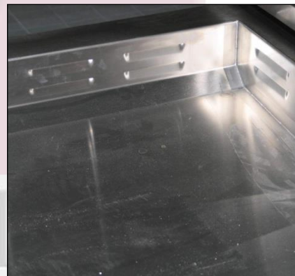
Unique MEDIS MT side wall downdraft extraction system (standard feature). Note: there is no air extraction whole in the plenum of the large sink below the work area!
