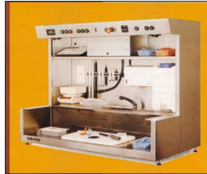
MA-0870 GrossLab (standard version). Equipped with several options
